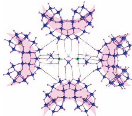
Figure 2. 2D representation of connectivity of the cluster showing the building units in 1a . The cluster is shown in ball-and-stick mode. The \{W_{29}Se_2\} branches are shown under crescent-shaped shadow (Fe, green; O, rose; Se, lime; W, blue). The links between building blocks are shown as dashed lines and are exaggerated longer to avoid overlapping of the four “crescent” subclusters. The cations are omitted for clarity.
